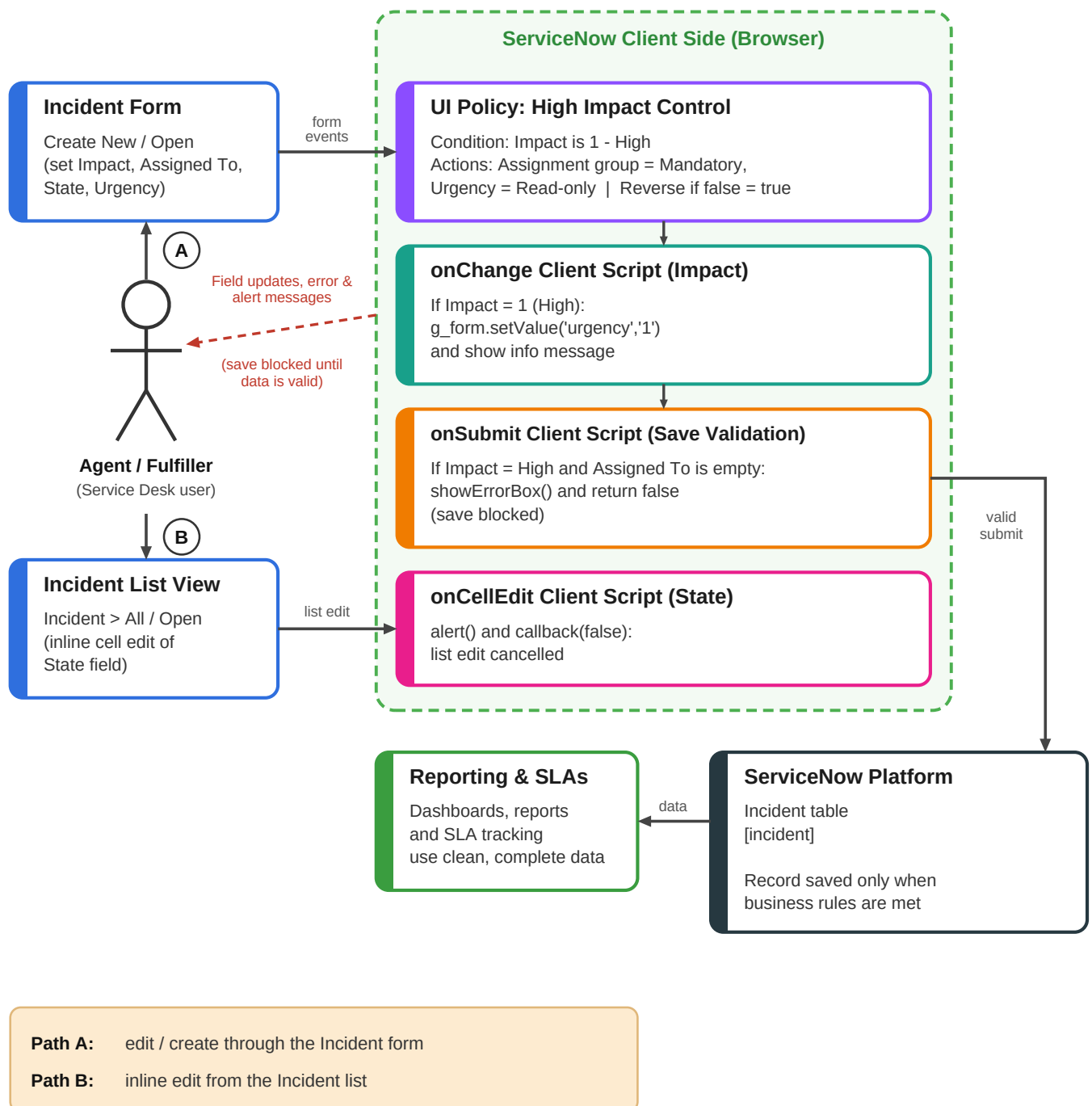
Figure 1: Architecture and data flow of the Incident client-side validation (UI Policy and Client Scripts) in ServiceNow
